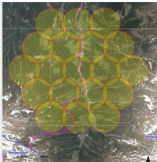
Figure 7: Stall new property
