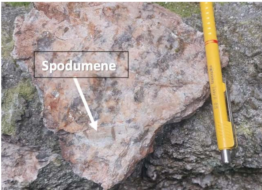
Figure 3: Spodumene occurrence from the Sankt Rad project
