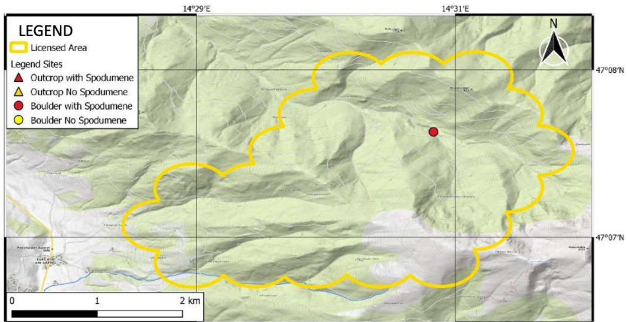
Figure 6: Legend property spodumene occurrences
