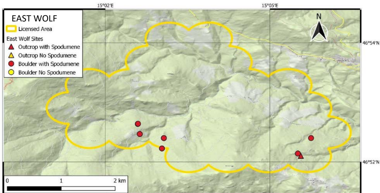
Figure 4: Pegmatites and spodumene occurrences on the East Wolf property
